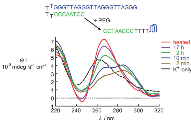
Figure 1. G-quadruplex formation and structural transition in a DNA duplex carrying the core telomere sequence G 3 (T 2 AG 3 ) 3 at the 3' end monitored by CD spectroscopy. The DNA hairpin originally formed in a 150 mM K + buffer converted into a G-quadruplex when the sample was mixed with an equal volume of the same buffer containing 80% (w/v) PEG 200. CD spectra were collected at the indicated time after mixing at 37 °C. PEG = poly(ethylene glycol).
